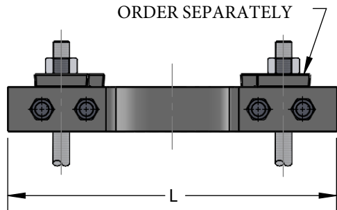
FIG. 599 WASHER ORDER SEPARATELY
