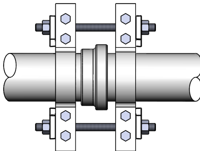
TYPICAL INSTALLATION
