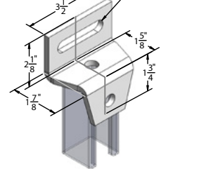
9065ZF adjustable offset gusseted "z" support
