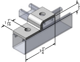
9061ZF 2-hole "z" support for 1-5/8" x 1-3/8" strut
