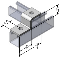
9063ZF 2-hole "z" support for 1-5/8" x 2-7/16" strut
