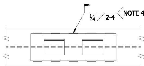
PAD WELD DETAIL
