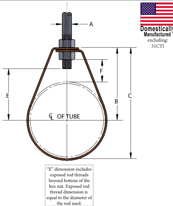
FIG. 31CT band hanger for copper tubing
