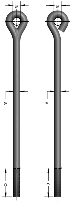
Welded FIG. 26W
