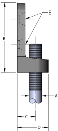
FIG. 155 steel beam clamp
