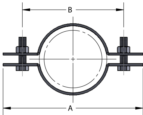
FIG. 48 riser clamp for plastic pipe
