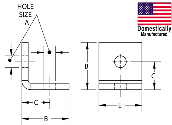
FIG. 53 angle bracket
