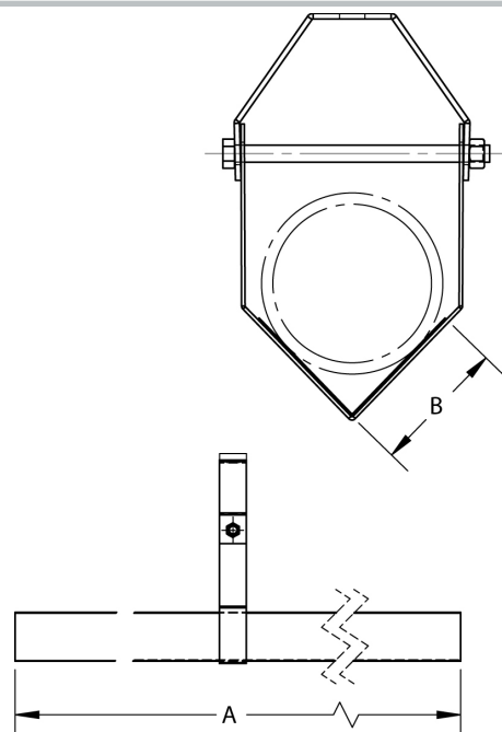
FIG. 12 v-channel
