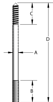
FIG. 55 hanger bolts
